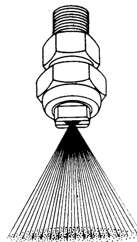
Figure 1. Regular Flat-Fan.
