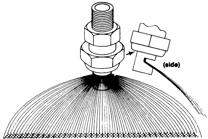
Figure 4. Flooding Flat-Fan.
